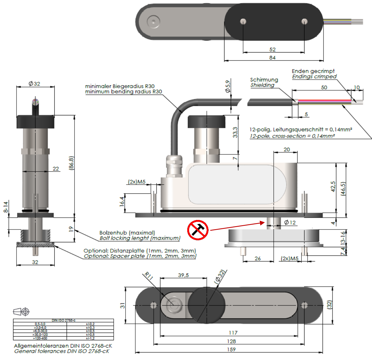
Figure 2 Product Drawing
