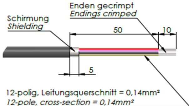
Figure 7 Connection lead
